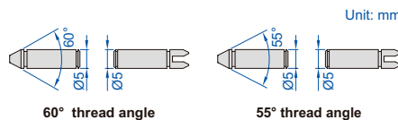
60° thread angle
