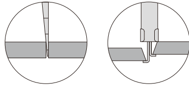
fit-up gap internal misalignment
